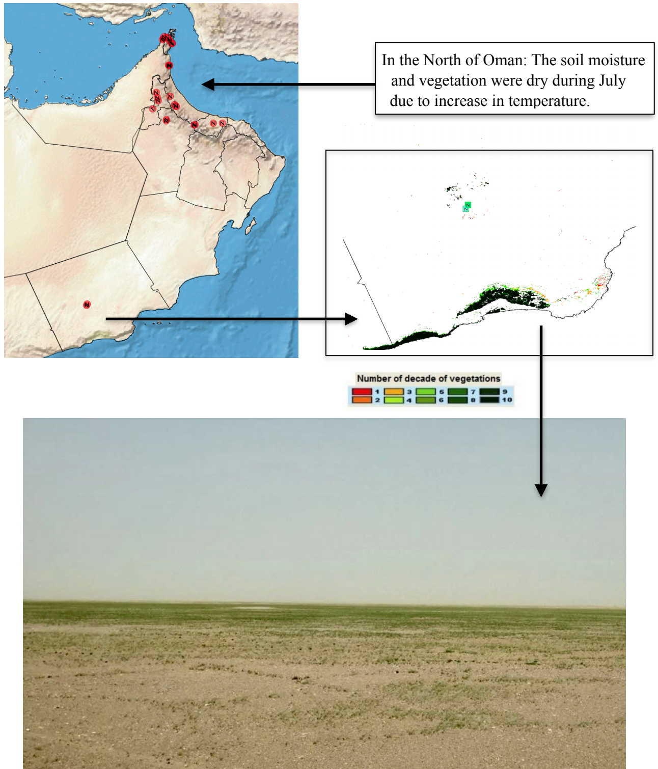
Fig 1. Desert Locust situation during July 2018 with RAMSES Map and Greening Image during 2 nd decade of July 2018. The arrow indicates the Dhofar Governorate where heavy rains fell in the last May. It shows that the vegetation started to be green. The greening of vegetation have started in appear in Thamreat plains.
