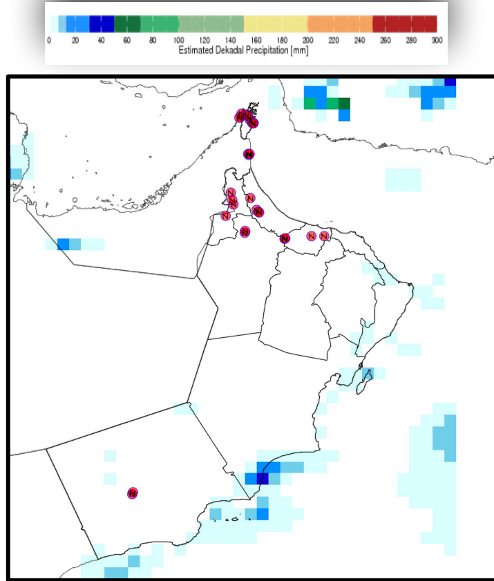
Fig 2. Rainfall estimation during 1st decade July 2018. No locust has been seen in all surveyed sites. The survey operations have showed that the soil moisture was dry (red dots) in all surveyed locations located at North, and also at the South of Oman (Dhofar).
